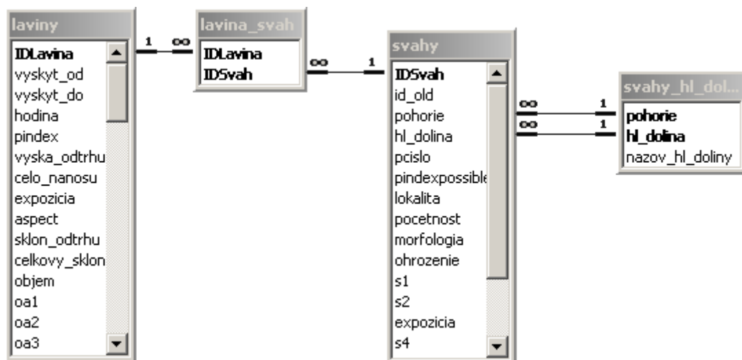
Fig. 3: Relationships among the core tables in SLPDB.
