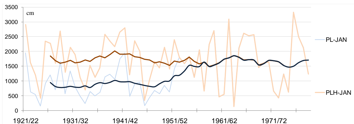
Fig. 15: January mean snow depths and 11-year running averages from Partizánska Ľupča – Magurka, PL-JAN unadjusted and PLH-JAN adjusted.
