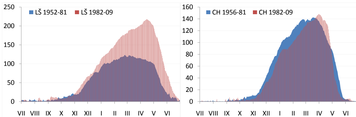
Fig. 16: Annual course of snow depth [cm] at the Lomnický štít (LŠ) and Chopok (CH) stations. Note the different shapes in two successive averaging periods and shifting of annual maxima.
