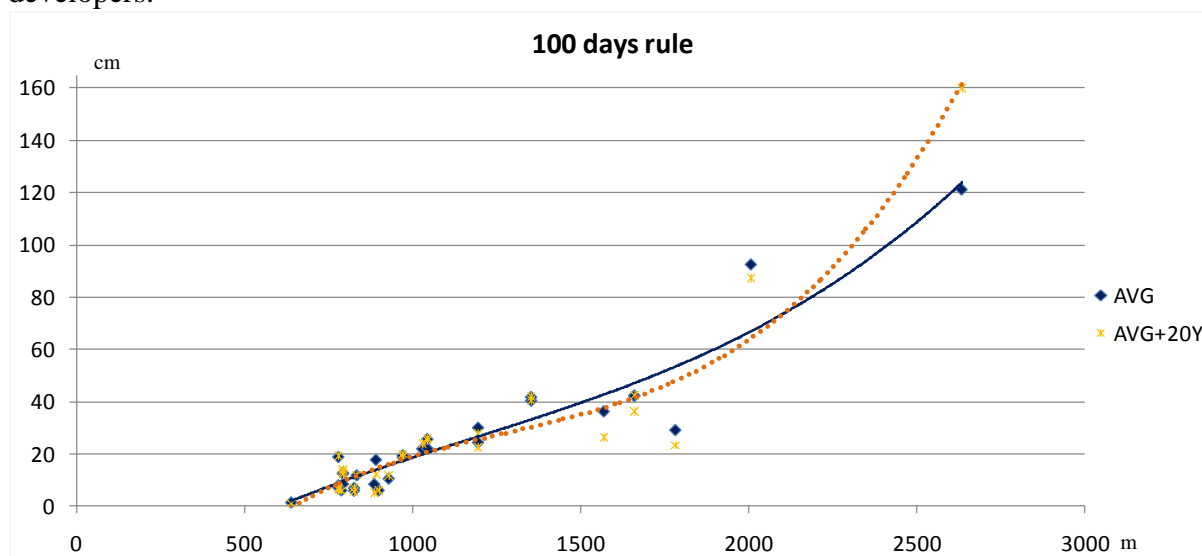
Fig. 20: The 100-days-rule characteristic and the dependence on altitude. The full line is a polynomial fit of the current average (AVG). The dotted line represents a change on the 20-year-horizon, if the trends are applied.
