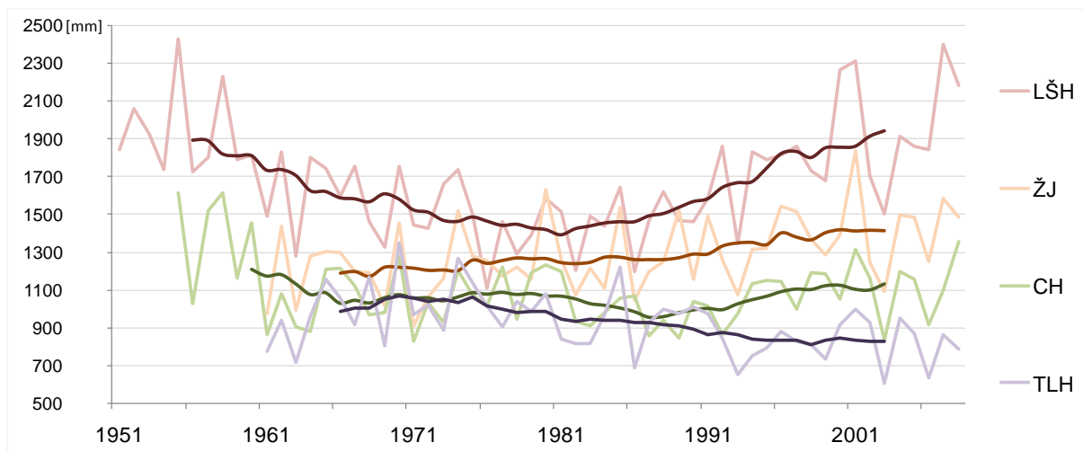
Fig. 10: Yearly sums of daily precipitation totals [mm] and 11-year running averages from the Lomnický štít (adjusted), Ždiar-Javorina, Chopok (adjusted) and Šumiac stations.
