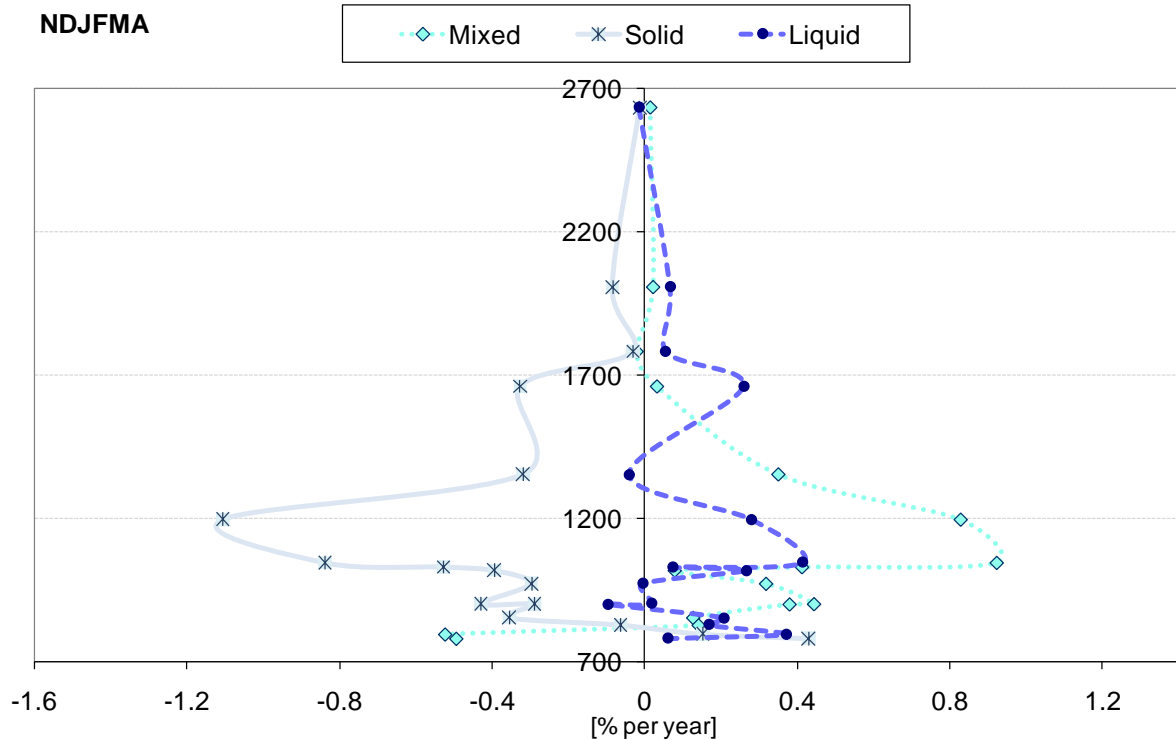
Fig. 22: Trends (1981/82–2007/08) of ratios of mixed (M), solid (S) and liquid (L) precipitation to the total precipitation amount from November to April (NDJFMA) for selected meteorological stations above 700 m.
